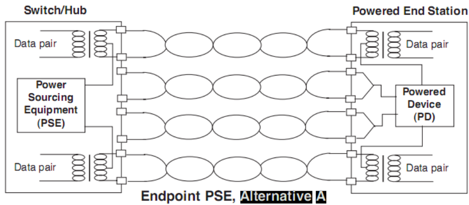
Figure 9 PoE Technology
