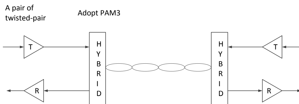
Figure 5 2D-PAM3 Encoding
