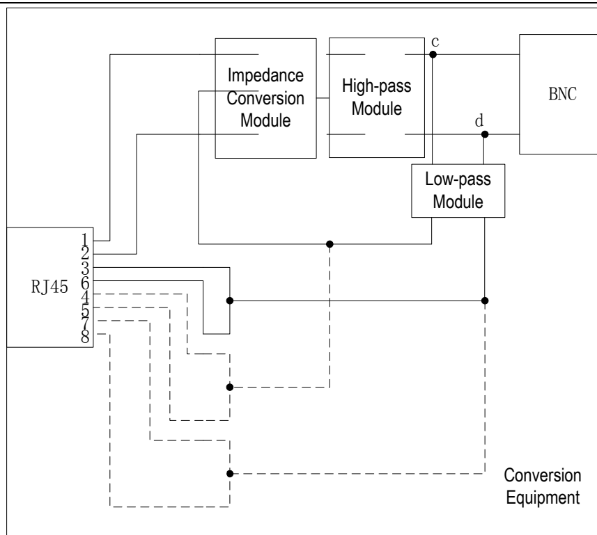
Figure 10 PoC Technology
