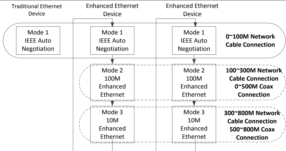
Figure 8 Mode Negotiation
