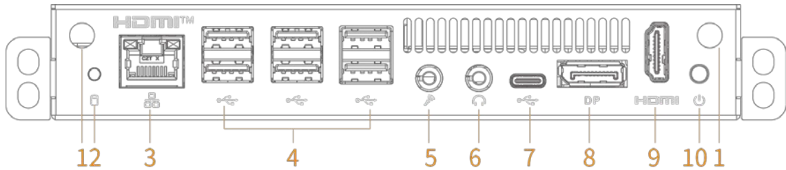
Figure 2-1 Front panel
